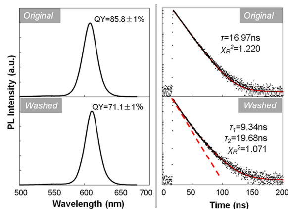
Figure 9. PL spectra (left panel) and PL decay kinetics (right panel) of zinc-blende core/shell nanocrystals with 4 monolayers of CdS shell before (top) and after (bottom) washing to remove some of the surface ligands. The red solid line (red dashed line) is the fitting results for the entire data series (for the first few data points). The PL QY was based on at least 10 different measurements for each sample.
