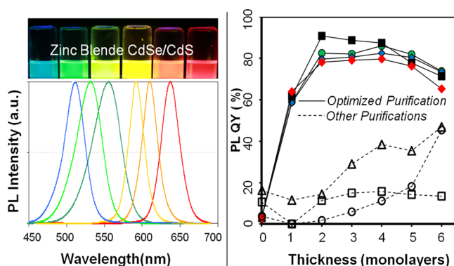
Figure 3. Left panel: Luminescence pictures under UV excitation (top) and PL spectra of zinc-blende CdSe/CdS core/shell nanocrystals with different emission wavelengths. Right panel: PL QY versus shell thickness for zinc-blende core and core/shell nanocrystals synthesized under different conditions. The experiments related to filled symbols in the plot were repeating synthetic runs using the optimized core purification procedure developed by this work (see text), and those associated with open symbols in the plot were carried out using other purification procedures (open squares, three times the hexane-methanol extraction; open triangles, acetone precipitation after three times of hexane-methanol extraction; and open circles, three times hexane-methanol extraction with the addition of fatty amines but without tributylphosphine).
